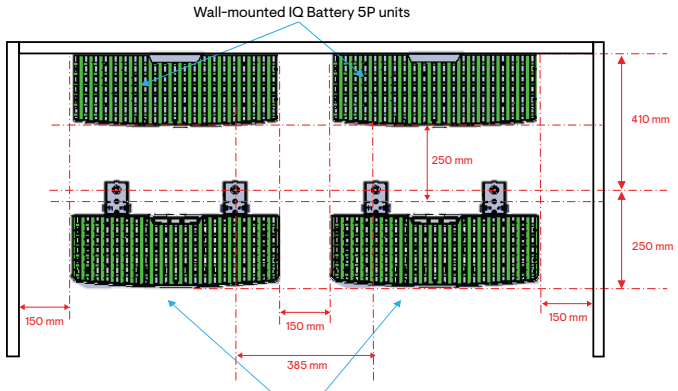
Pedestal-mounted IQ Battery 5P units Pedestal Mount spacing details: Top view
