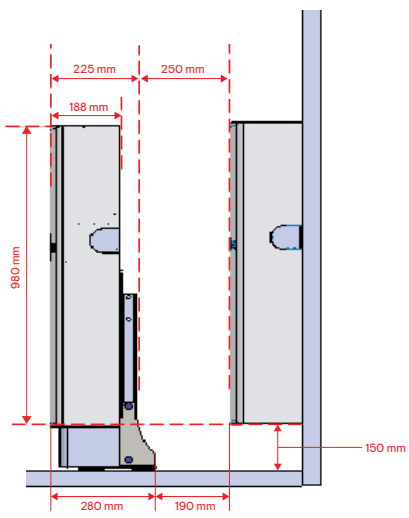
Minimum distance from the floor to the bottom of the unit (for both floor-mounted and wall-mounted)
